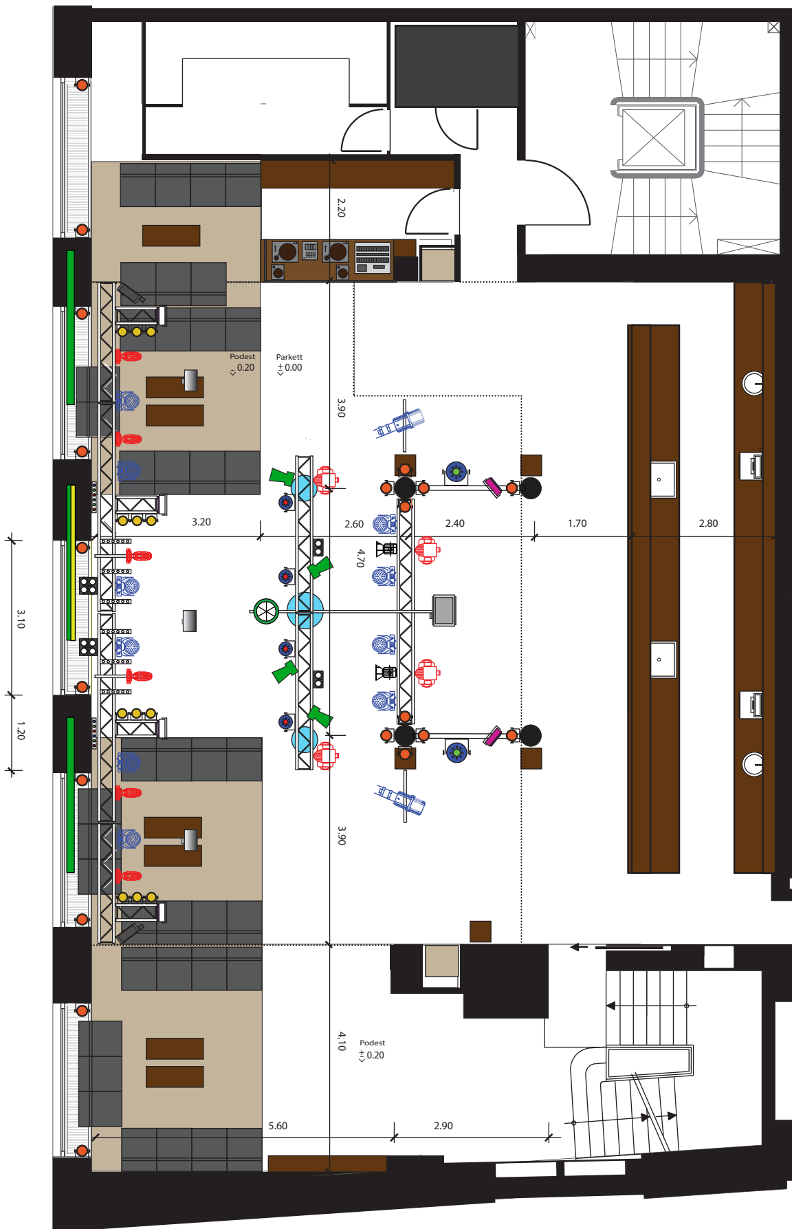
LAYOUT MAINFLOOR - CLUB
